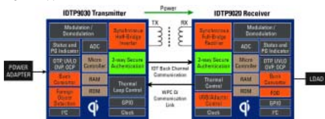
Figure 1: Wireless Charger System: Transmitter and Receiver Block Diagrams
