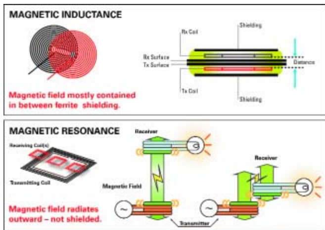
Figure 4: Magnetic fields
