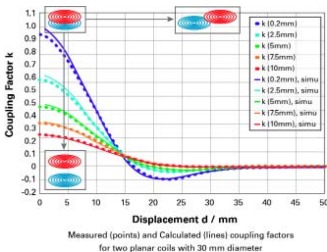
Figure 2: Coupling Displacement
