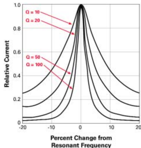
Figure 3: Q-factor percentage
